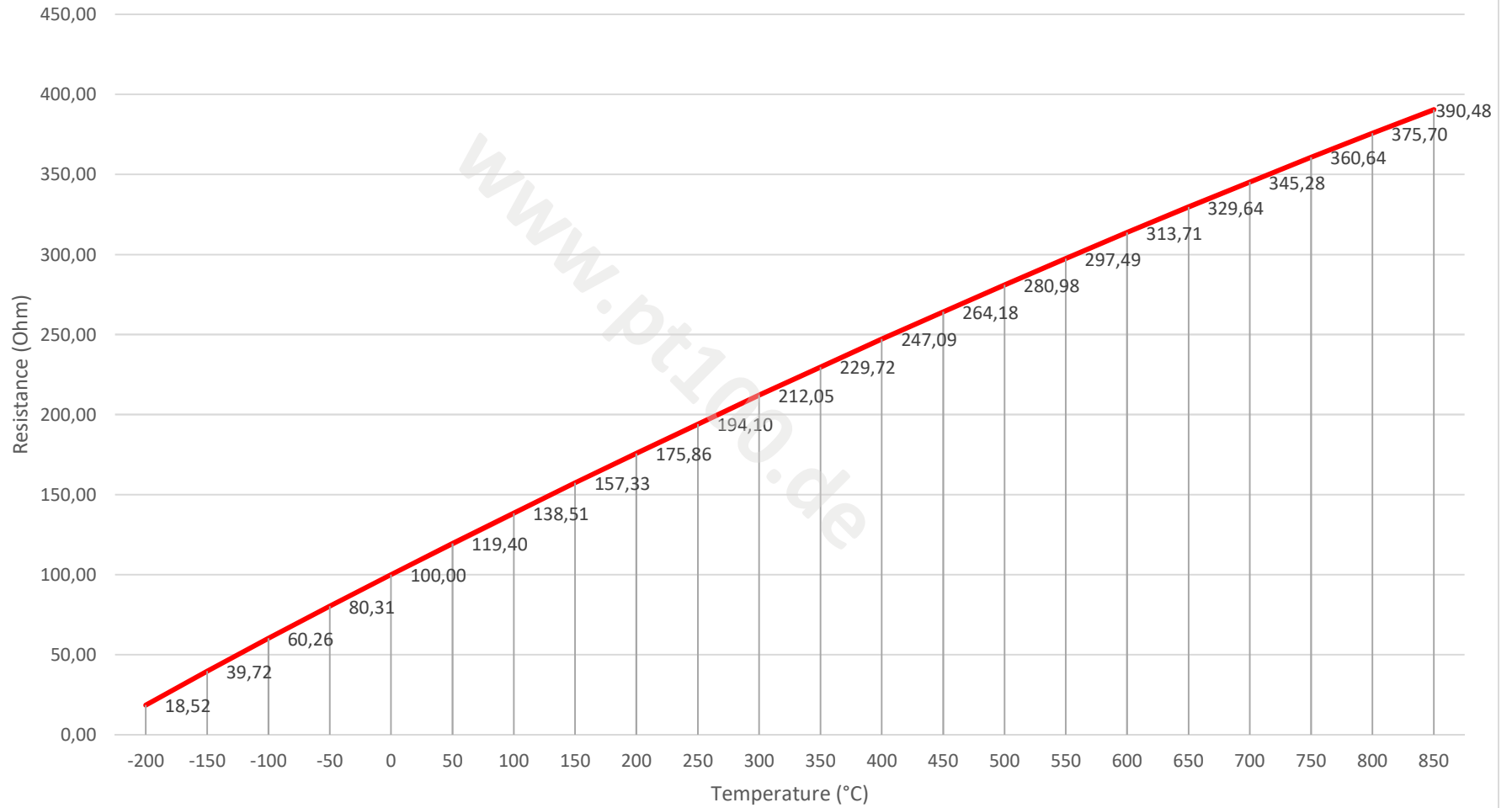
Pt100- resistance depending on temperature
