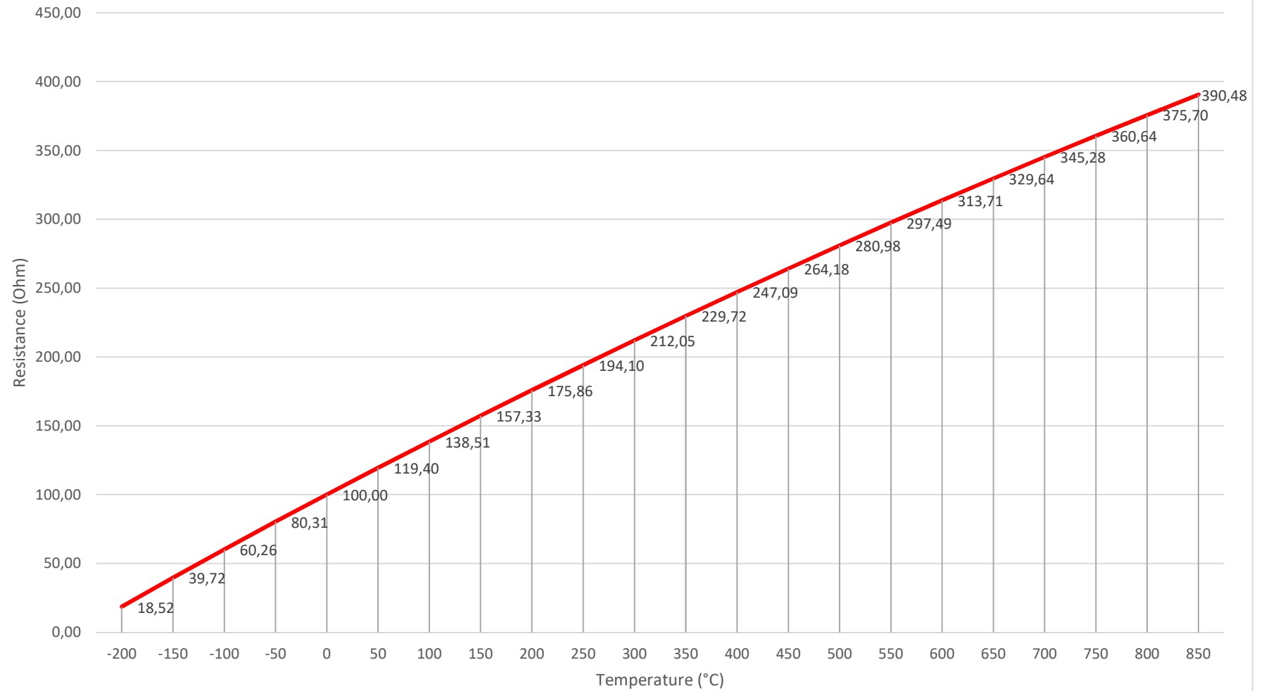
Pt100- resistance depending on temperature
